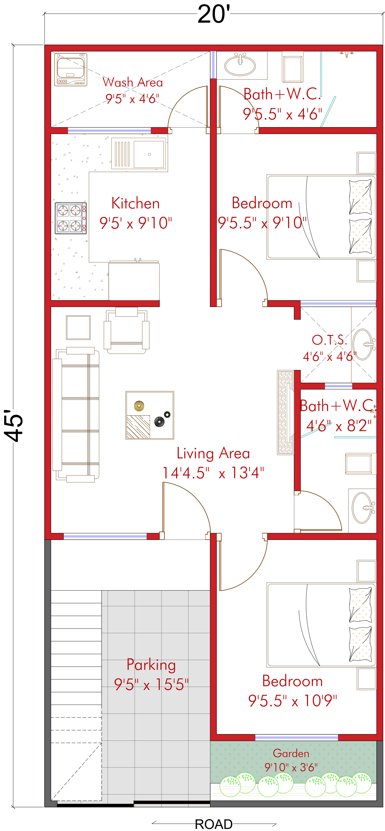
GROUND FLOOR PLAN 20'x45' House Design
