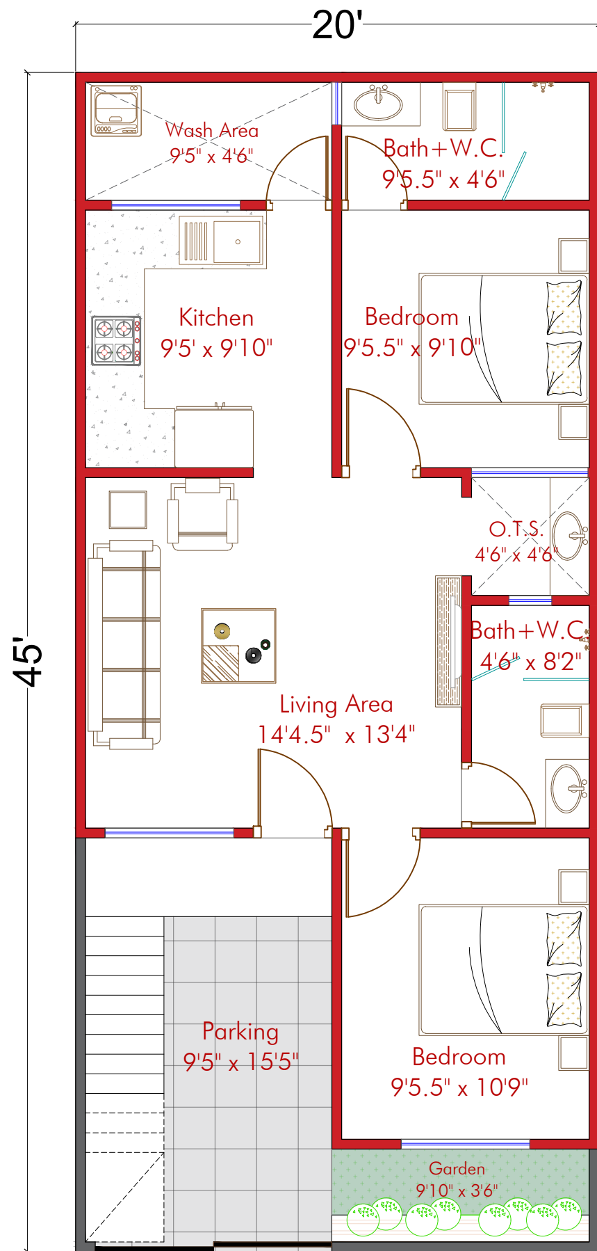
GROUND FLOOR PLAN 20'x45' House Design
