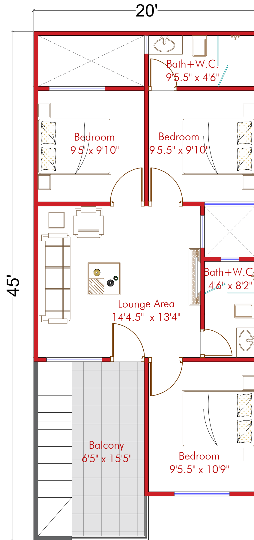
FIRST FLOOR PLAN 20'x45' House Design
