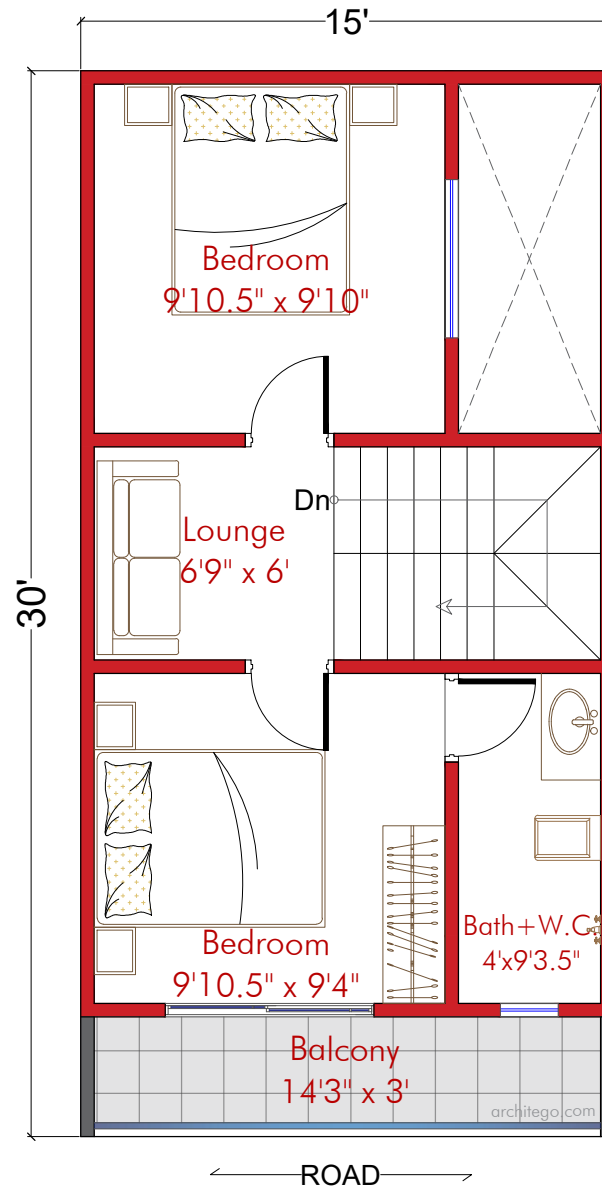
FIRST FLOOR PLAN 15'x30' House Design
