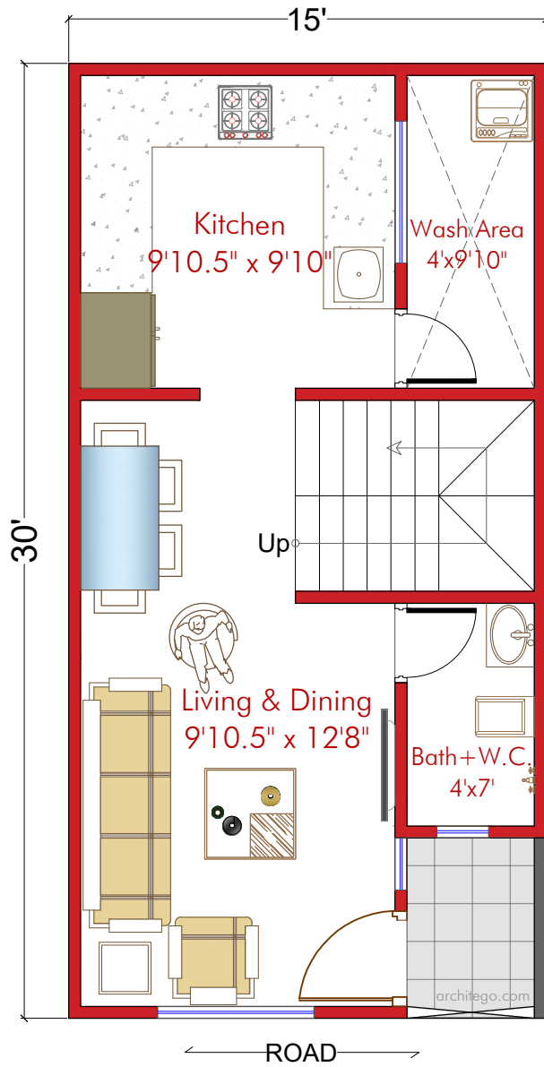
GROUND FLOOR PLAN 15'x30' House Design
