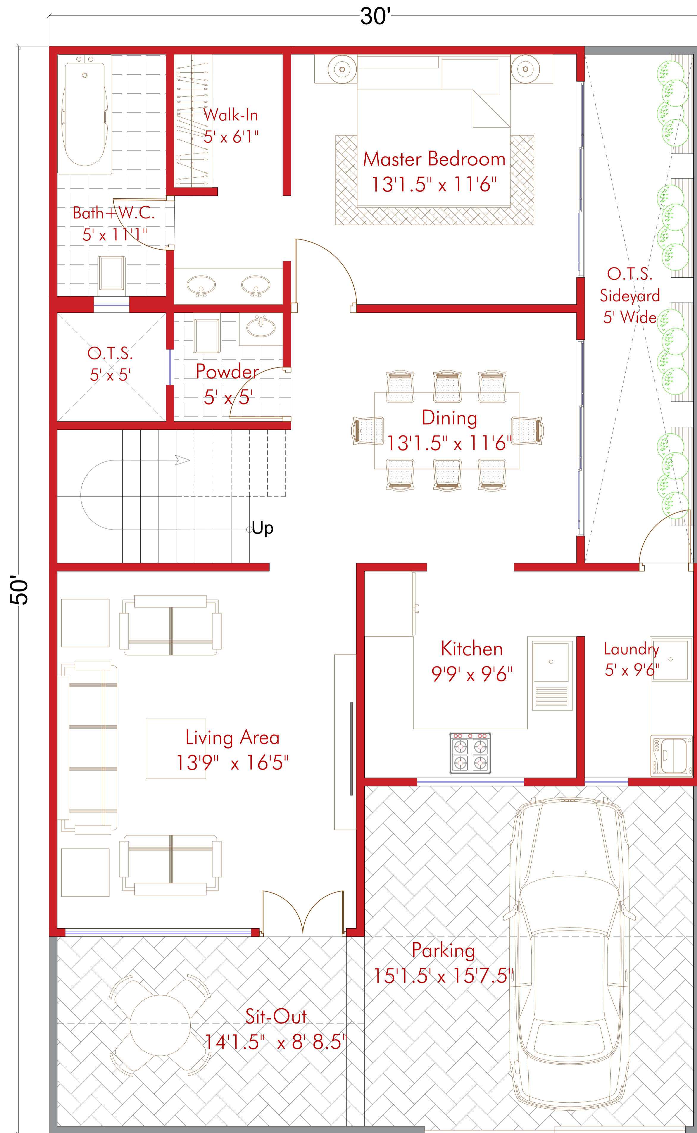
GROUND FLOOR PLAN 30'x50' House Design
