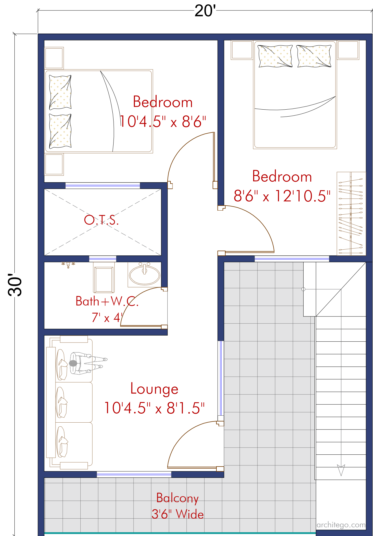
FIRST FLOOR PLAN 20'x30' House Design
