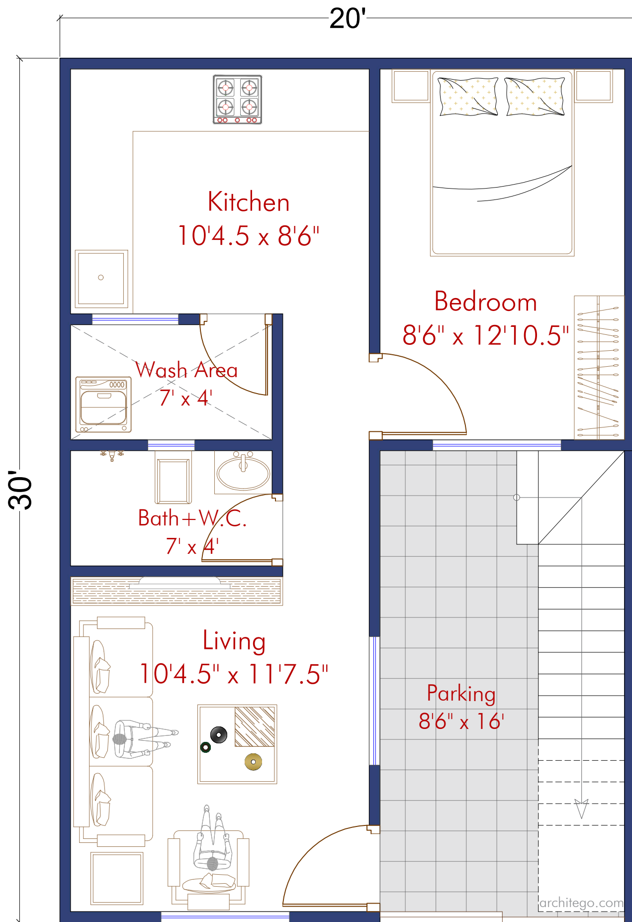
GROUND FLOOR PLAN 20'x30' House Design
